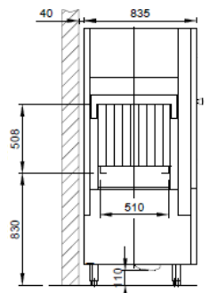
ELEVATION VIEW A
